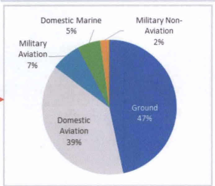
Figure 3-6: 2017 Transportation Emissions by End-Use Sector
