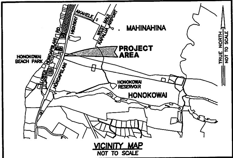
SKETCH SHOWING EASEMENT D FOR ACCESS AND UTILITY PURPOSES AFFECTING GRANT S-15870 TO DEPARTMENT OF HAWAIIAN HOME LANDS AT HONOKOWAI, LAHAINA, MAUI, HAWAII
