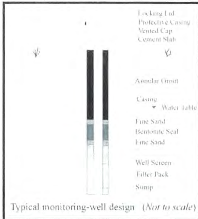
Figure 2. Depiction of a Typical Piezometer Installation
