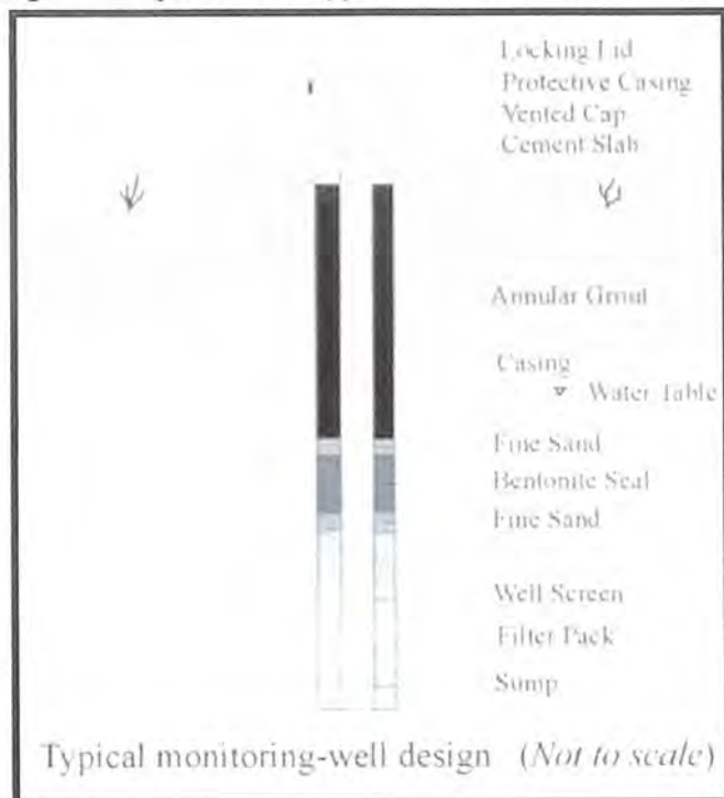
Figure 2. Depiction of a Typical Piezometer Installation
