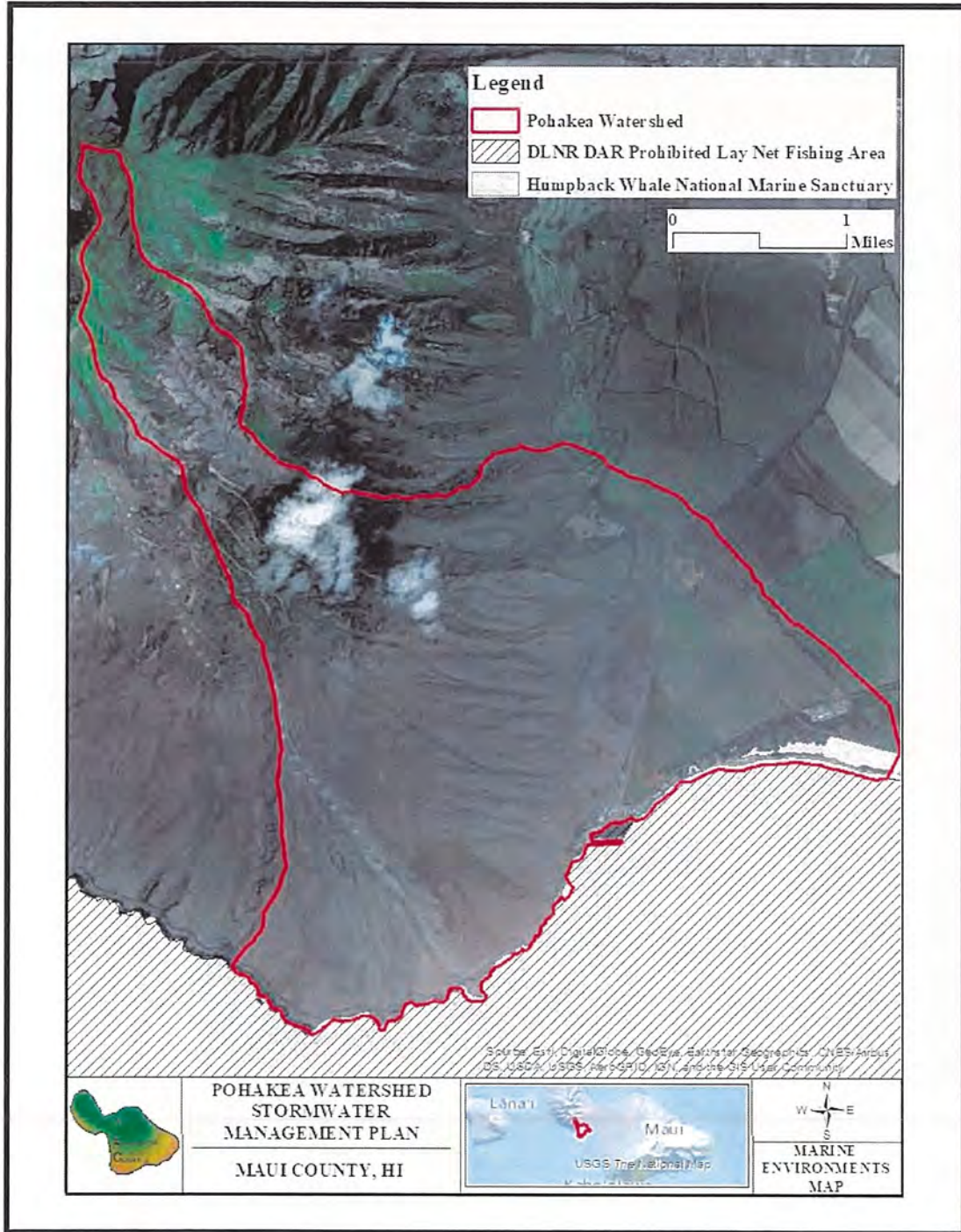
Figure 8. Marine Environments
