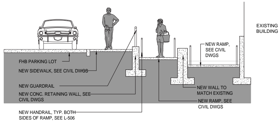
SECTION - RAMP (BASE BID FHB PARKING LOT)
