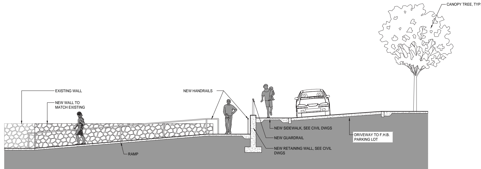
SECTION - RAMP (BASE BID FHB PARKING LOT)
