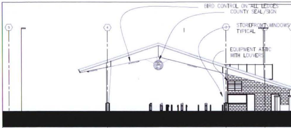
2 WEST ELEVATION
