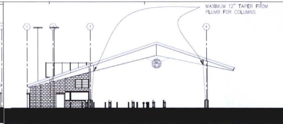
1 EAST ELEVATION
