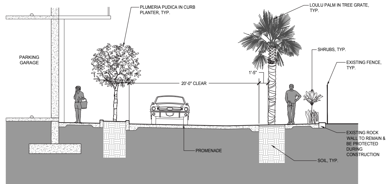
SECTION - SHARED PROMENADE BASE BID ROAD A
