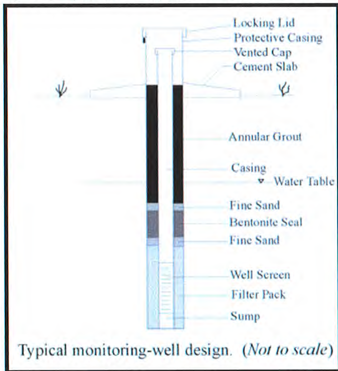
Figure 2. Depiction of a Typical Piezometer Installation
