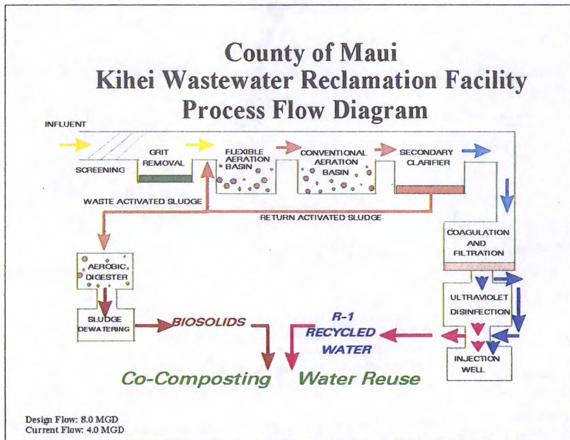
Figure 2: Kihei WWRF Process Flow Diagram
