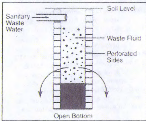
Figure 7: Cesspool
