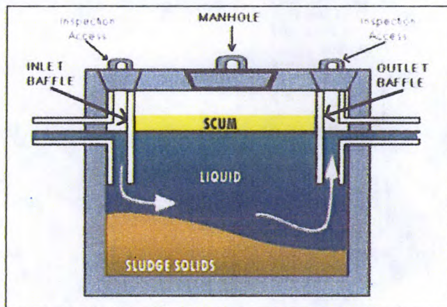
Figure 8: Septic Tank
