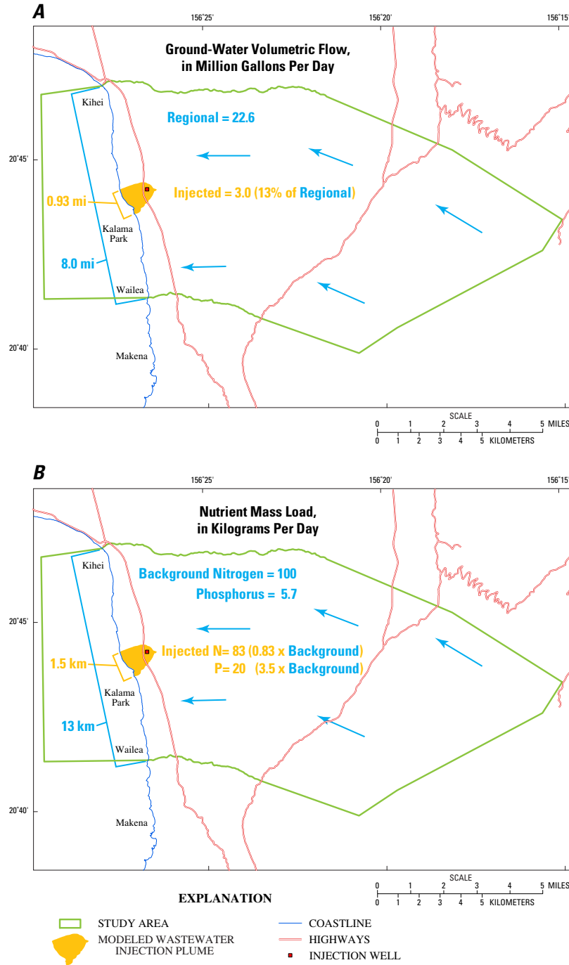
Figure 19. Maps showing estimated ground-water and nutrient fluxes, Kihei, Hawaii. Blue lettering denotes regional fluxes and yellow denotes injected fluxes. A , Recharge-driven regional flow (blue arrows) discharges along 8.0 miles of coast; injected effluent discharges from a 0.93-mile-wide plume and is 13 percent of regional flow. B , Injected nitrogen and phosphorus loads are 0.83 and 3.5 times background load in regional flow. C , Injected nitrogen and phosphorus fluxes (load per length of coast) are 7.1 and 30 times background flux. D , Natural attenuation in the aquifer reduces injected nitrogen and phosphorus fluxes to 3.5 and 3.4 times background by the time effluent reaches the downgradient well.
