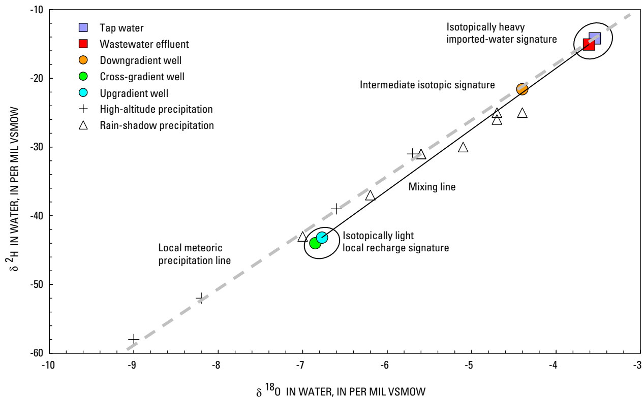
Figure 15. Graph showing oxygen and hydrogen stable-isotope compositions in tap water, wastewater effluent, and untreated ground water, Kihei, Hawaii. The isotopic composition of imported tap water is distinctly heavier than that of local ground water from the upgradient and cross-gradient wells; this signature is modified little during use and treatment and persists in wastewater. The downgradient well has an intermediate composition that is closer to tap water and wastewater than to local ground water. VSMOW (Vienna Standard Mean Ocean Water) is a reference standard that is used to express isotopic compositions. (Precipitation data and meteoric line from Scholl and others, 2002.)
