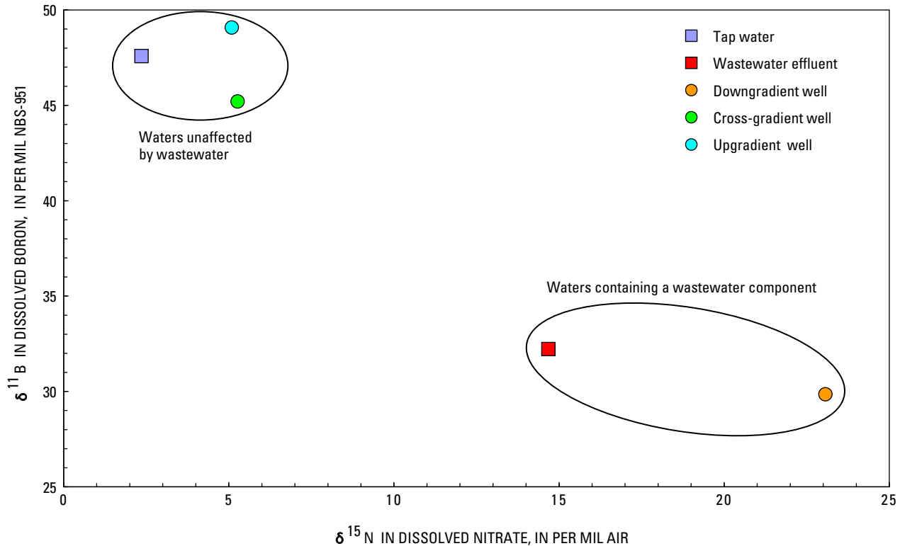
Figure 18. Graph showing boron and nitrogen stable-isotope compositions in tap water, wastewater effluent, and untreated ground water, Kihei, Hawaii. Boron-isotope composition is distinctly lighter in wastewater and the downgradient well than in imported tap water and in local ground water from the upgradient and cross-gradient wells. NBS-951 (National Bureau of Standards) and AIR (atmospheric air) are reference standards that are used to express isotopic compositions.
