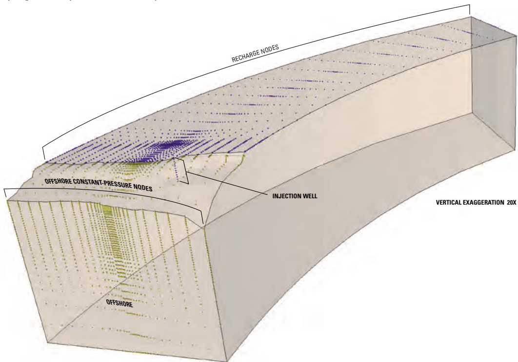
Figure 21. Block diagram showing the model finite-element mesh, Kihei, Hawaii. View is to the northeast. The model has 37 layers of elements, and vertical mesh spacing is finest at the top and progressively coarser with depth.
