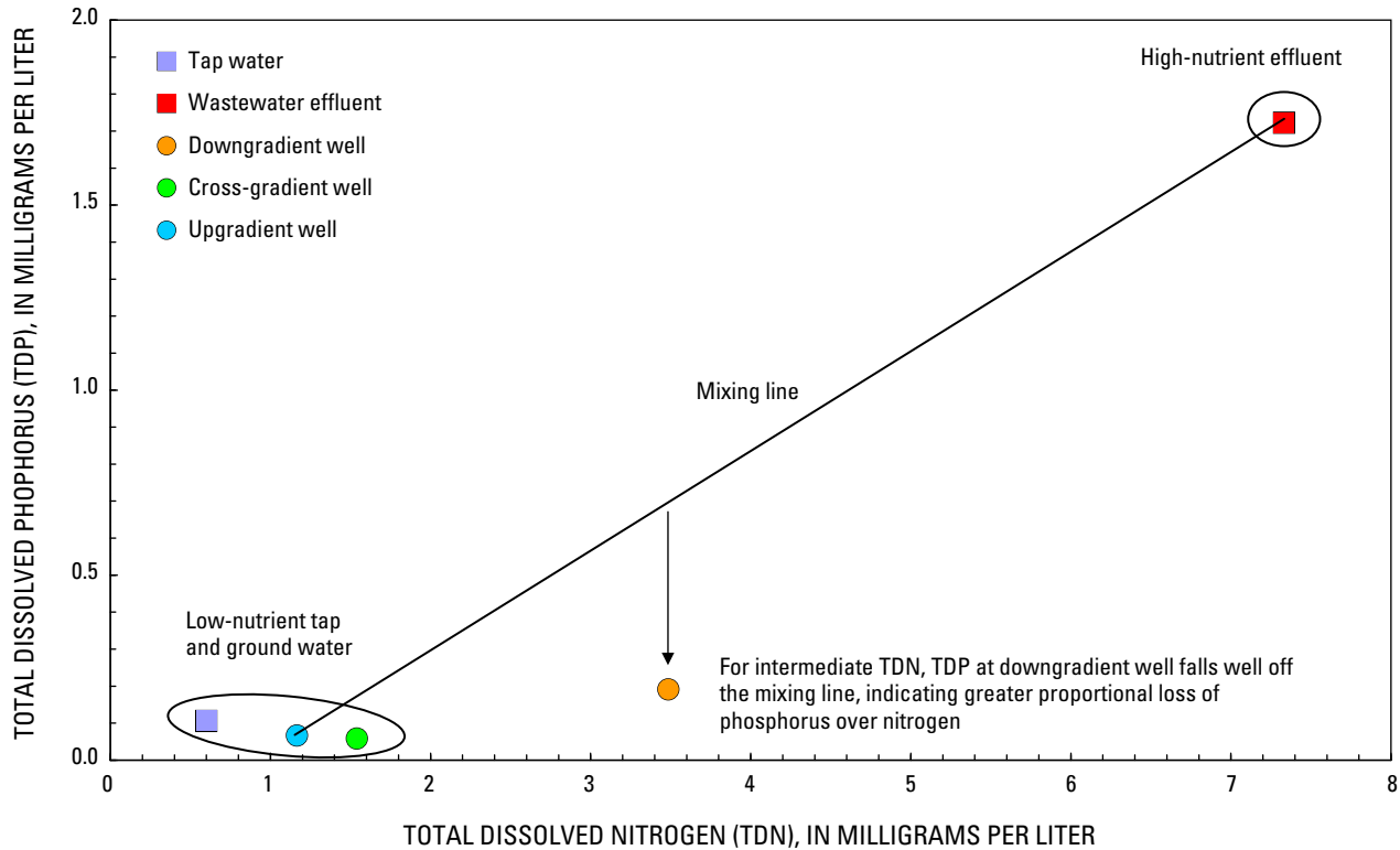
Figure 14. Graph showing dissolved nitrogen and phosphorus concentrations in tap water, wastewater effluent, and untreated ground water, Kihei, Hawaii. Wastewater effluent is much higher in nutrients than imported tap water and local ground water from the upgradient and cross-gradient wells. Nutrient concentrations at the downgradient well are intermediate between wastewater and the other waters.
