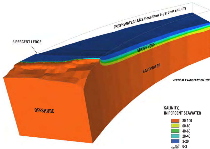
Figure 23. Block diagram showing modeled salinity for the natural recharge scenario, Kihei, Hawaii. View is to the northeast. Water fresher than 3 percent seawater has been omitted from the diagram to delineate the freshwater lens as clear space; ground water shoreward of the “3 percent ledge” is brackish. Recharge drives ground-water flow from mountain to shore within the freshwater lens, entraining underlying saltwater in the mixing zone. Mixed water discharges at the coast, drawing saltwater into the aquifer from offshore to replace it and driving circulatory saltwater flow at depth.
