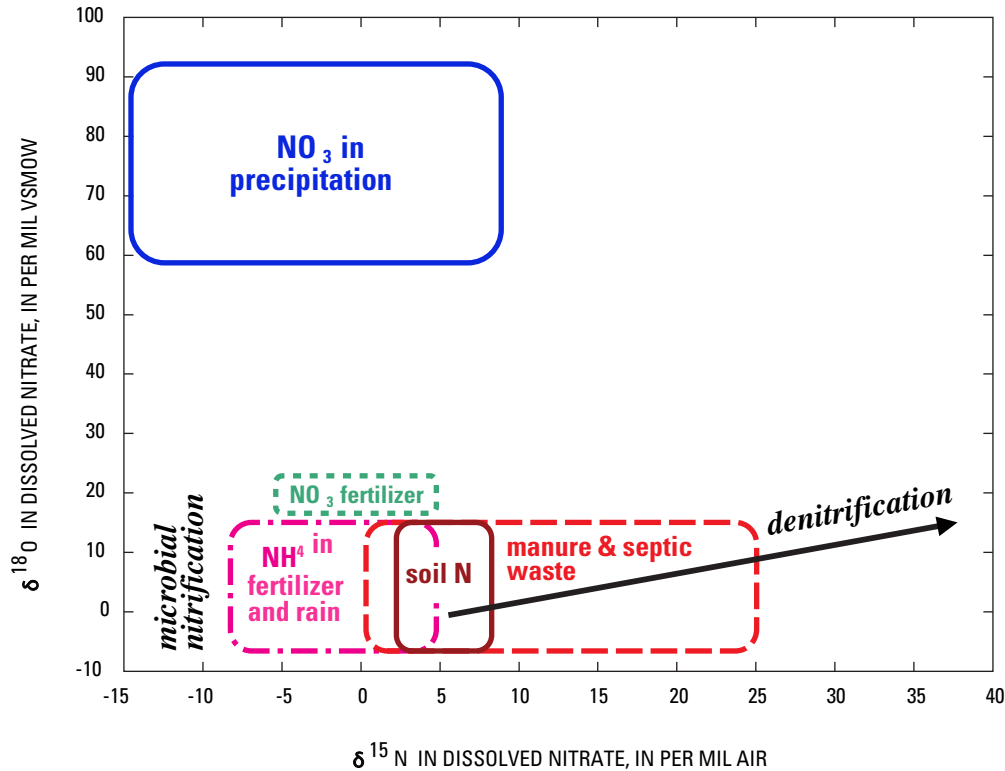
Figure 17. Graph showing nitrate source classification based on nitrogen and oxygen stable-isotope compositions in dissolved nitrate. Colored lines bound isotopic compositions of various nitrate sources and are based on results reported in many studies. Results from Kihei water samples fall within the soil and septic fields of this classification. VSMOW (Vienna Standard Mean Ocean Water) and AIR (atmospheric air) are reference standards that are used to express isotopic compositions. (Updated from Kendall and McDonnell, 1998, by Carol Kendall, USGS, written commun., 2006.)
