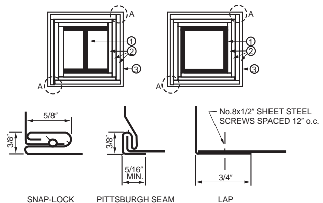
FIGURE 722.5.1(2) GYPSUM-PROTECTED STRUCTURAL STEEL COLUMNS WITH SHEET STEEL COLUMN COVERS
