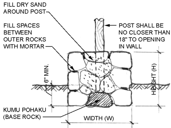
PĀA PŌOHAKU (FOUNDATION WALL)
